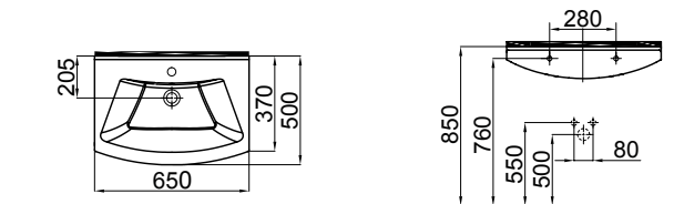
2801-0655 Vega Lavabo (50x65) Vega Furniture Washbasin
