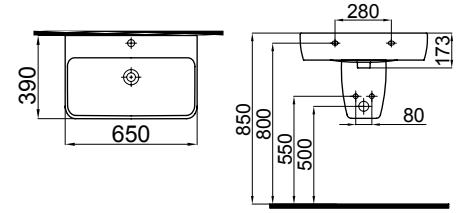
0101-0655 Lavabo / Washbasin (40x65) 3203-0000 Yarım Ayak / Half Pedestal (22x26x29)
